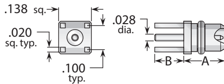
Figure 1 (Straight through-hole mount)
