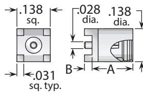
Figure 2 (Straight surface mount)
