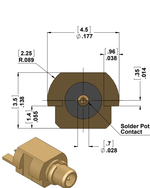
6068000G001-500 Fidelity+ Plug (Gold Plating)
