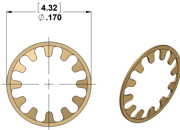
50-10019-01-AU Grounding Cage Spring Used on Fidelity+ Plugs/Males
