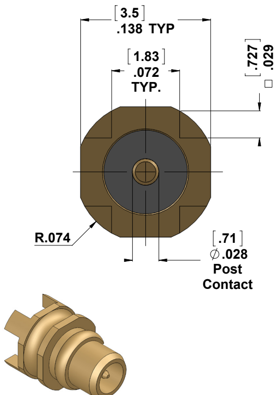
6068000G001-501 Fidelity+ Plug Low Profile Configuration (Gold Plating)
