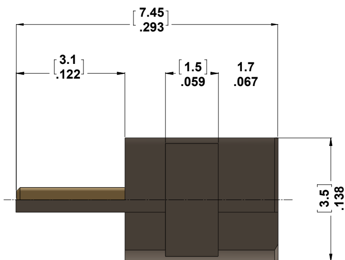
6067000N001-503 Fidelity+ Jack (Nickel Plating)
