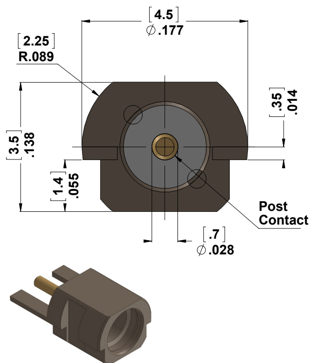
6067000N001-503 Fidelity+ Jack (Nickel Plating)
