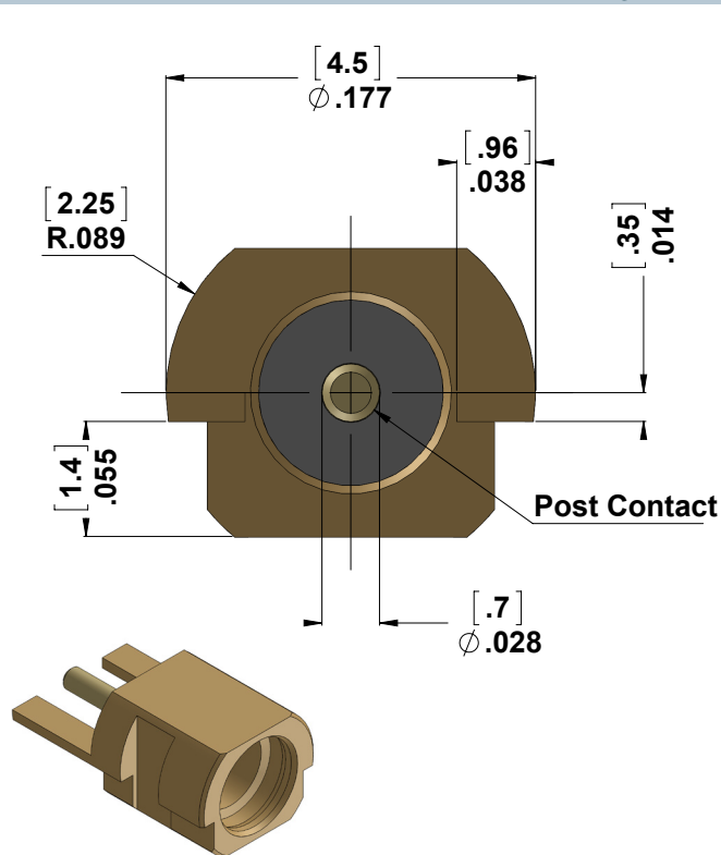
6067000G001-500 Fidelity+ Jack (Gold Plating)
