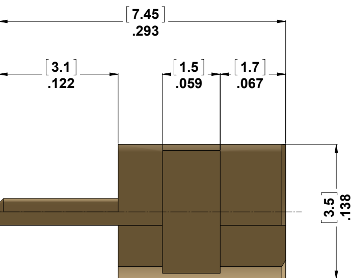
6067000G001-502 Fidelity+ Jack (Gold Plating)
