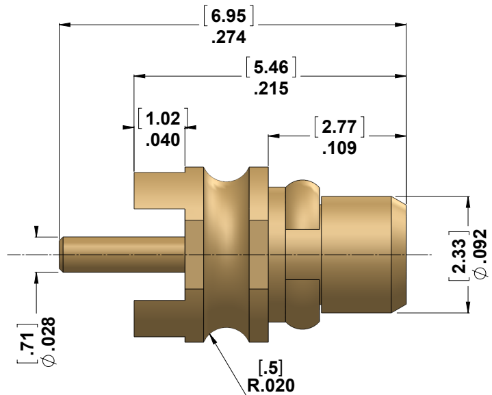
6068000G001-502 Fidelity+ Plug Low Profile Configuration (Gold Plating)
