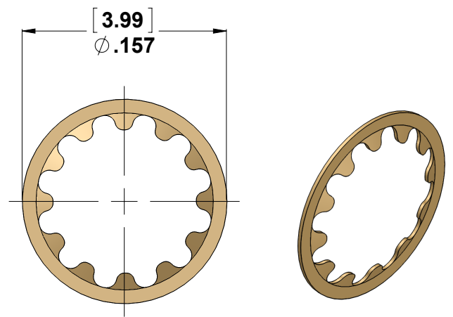
50-10020-01-AU Grounding Cage Spring Used on Fidelity+ Plugs/Males
