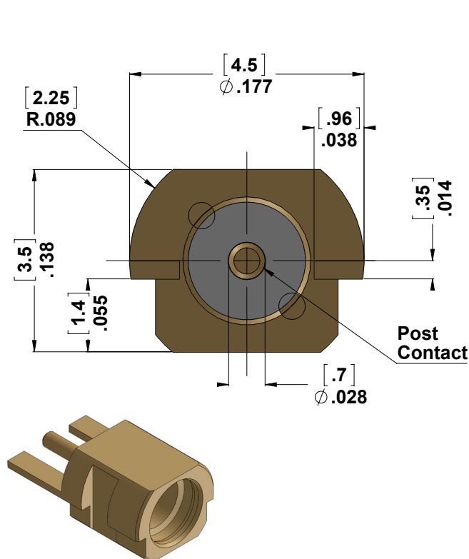
6067000G001-502 Fidelity+ Jack (Gold Plating)
