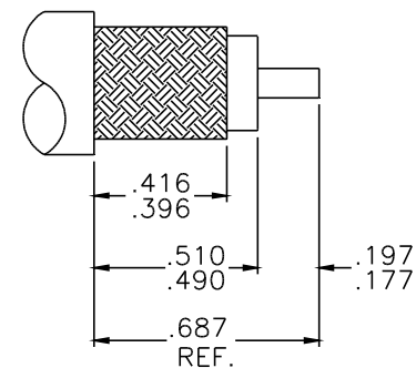
CABLE CUTTING DIMENSIONS
