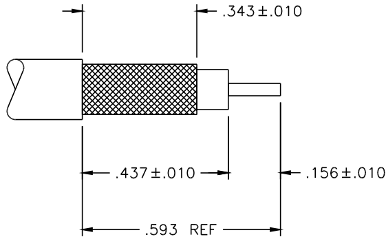
RECOMMENDED CABLE TRIMMING DIMENSIONS
