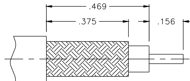
RECOMMENDED CABLE CUTTING DIMENSIONS
