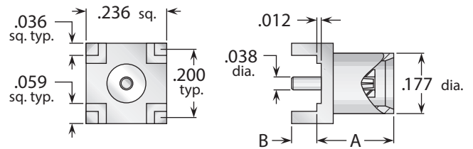
Figure 2 (Through-hole mount)
