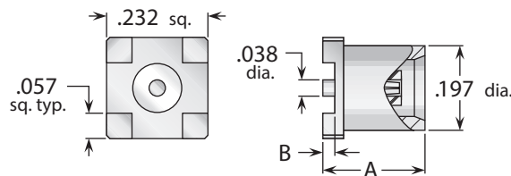
Figure 5 (Surface mount)
