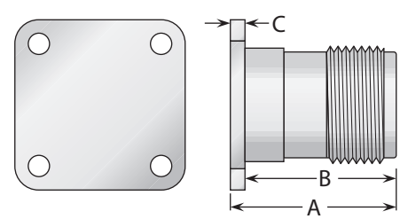
Figure 4 (Dummy receptacle)
