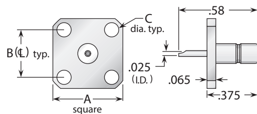
Figure 2 ( 1 / 2 " square flange)
