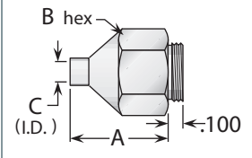
Figure 4 (Direct solder for semi-rigid cable)
