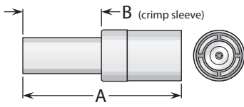
Figure 1 (Crimp type)
