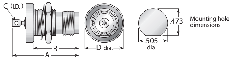
Figure 1 (Rear mount)
