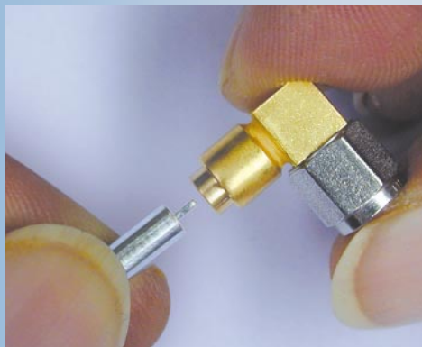
Trim cable and insert into connector.
