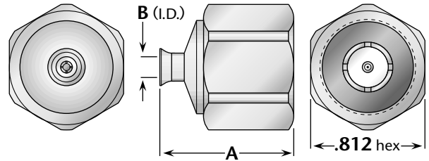
Figure 2 (Hex coupling nut)
